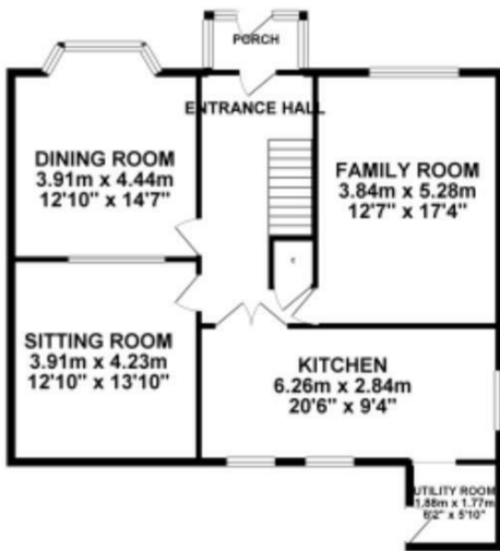
GROUND FLOOR 112.91 sq. m. ( 1215.38 sq. ft. )
